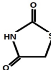
Figure 1: Thiazolidine -2, 4-dione.
